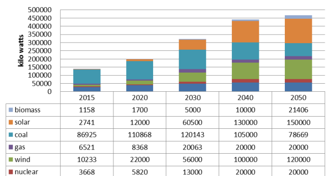
Fig. 3. Energy capacity prediction from 2015 to 2050.
