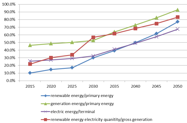
Fig. 4. Energy proportion comparison from 2015 to 2050.
